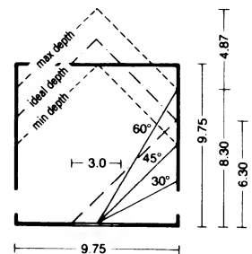
10 Exhibition room with side lighting
